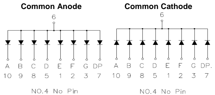
Figure 1. INND-TS40 series Internal Circuit Diagram
