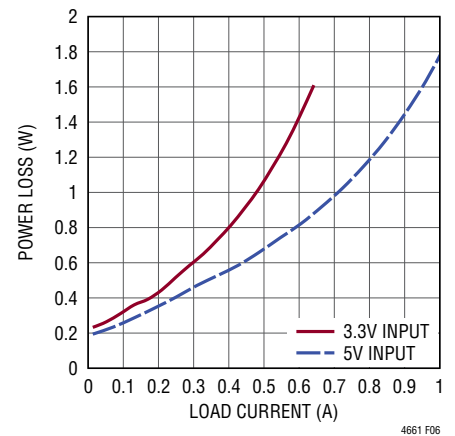
Figure 6. 12V Output Power Loss
