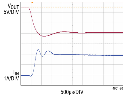
Short-Circuit Response
