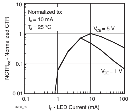
Fig. 5 - Normalized CTR vs. Forward Current
