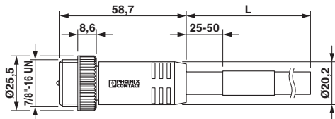
7/8"-16UNF plug, straight
