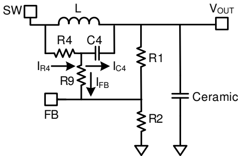
Figure 7: Simplified PWM-Mode Circuit with External Ramp Compensation
