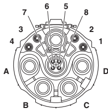
Pin assignment of socket signal, coding 1
