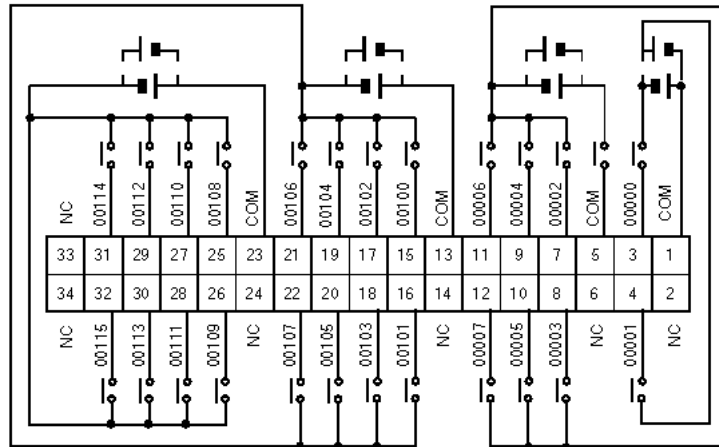
Input Connector
