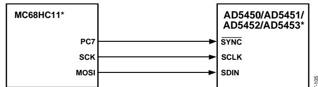
Figure 60. MC68HC11 to AD5450/AD5451/AD5452/AD5453 Interface
