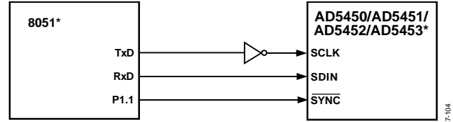
Figure 59. 80C51/80L51 to AD5450/AD5451/AD5452/AD5453 Interface
